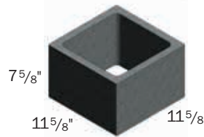
Column (C-12)
